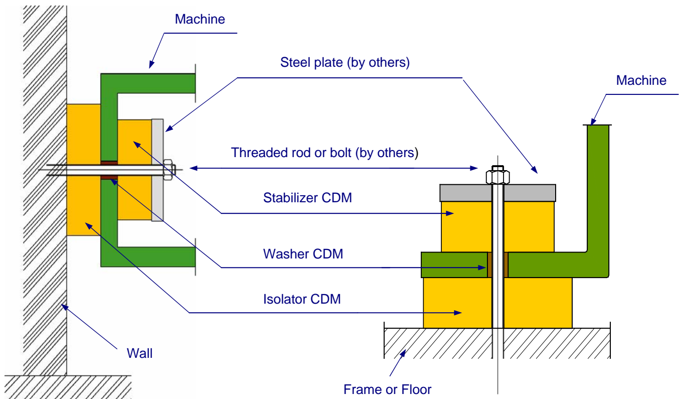
Horizontal and vertical CDM-ISO-MACHINE-FIX setup
