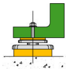
TYPE C Low horizontal forces Tunable in height
