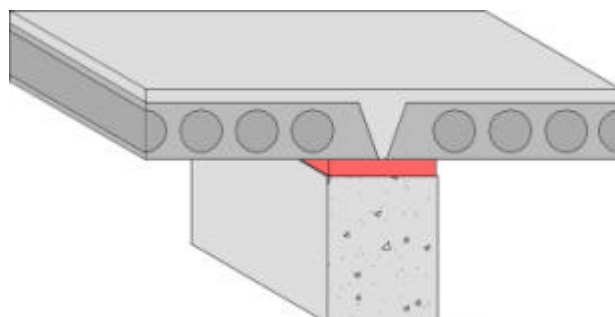
Decoupling of floor segments
