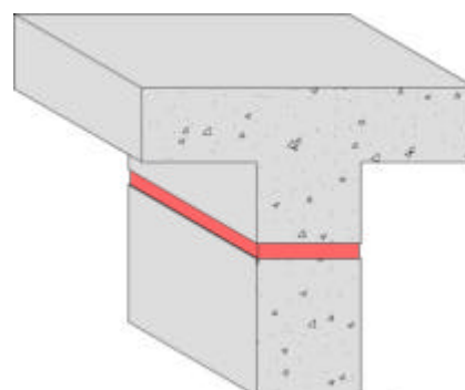
Decoupling of walls and beams
