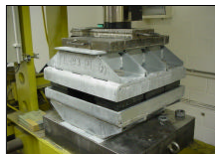
Box precompression
